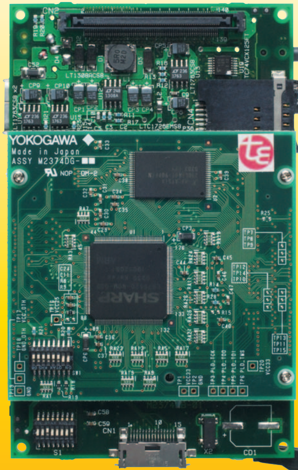
The CPU Board of the T-Engine/ARM720-LH7 Development kit (in full-scale)
