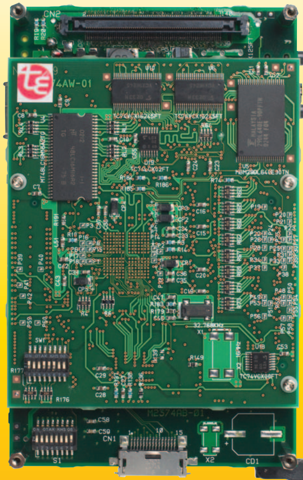
The CPU Board of the T-Engine/ARM920-MX1 Development kit (in full-scale)
