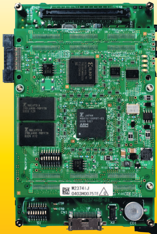
The CPU Board of the T-Engine/ARM926-MB8 Development kit (in full-scale)
