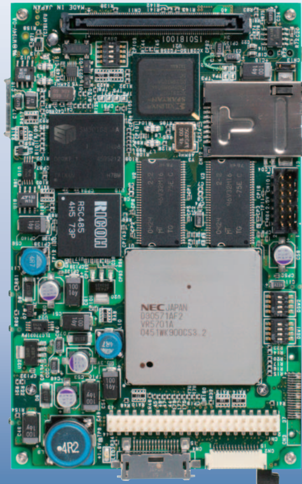
The CPU Board of the T-Engine/VR5701 Development kit (in full-scale)
